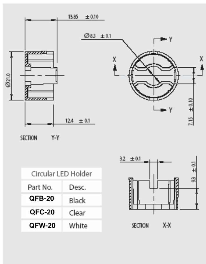
Fig. 1 BTH-QFX-20 Holders
