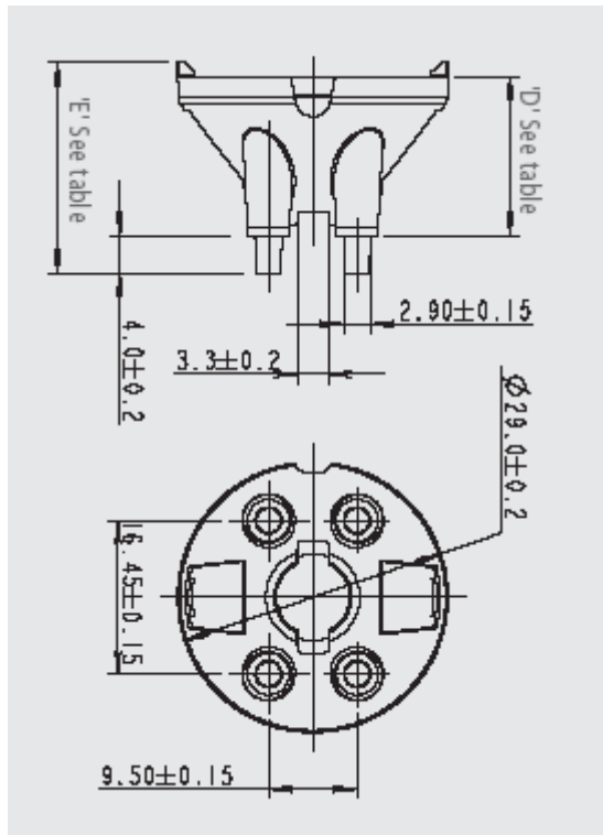
Fig.3 BTH-QFX-26-X Holder
