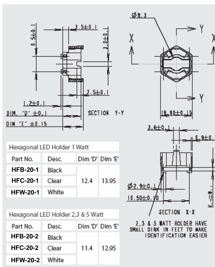
Fig. 2 BTH-HFX-20 Holders
