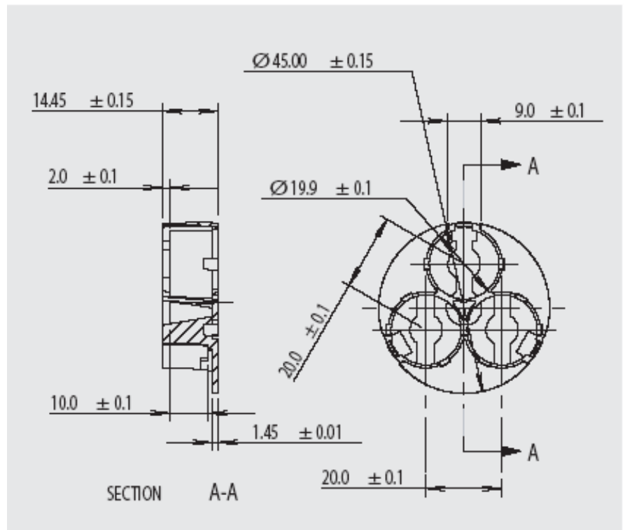
Fig.4 BTH-3QFX-20 Holder
