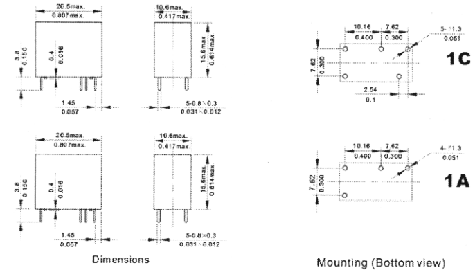
Mounting (Bottom view)
