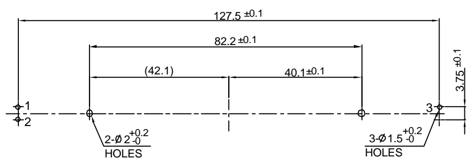
MOUNTING HOLE DETAIL
